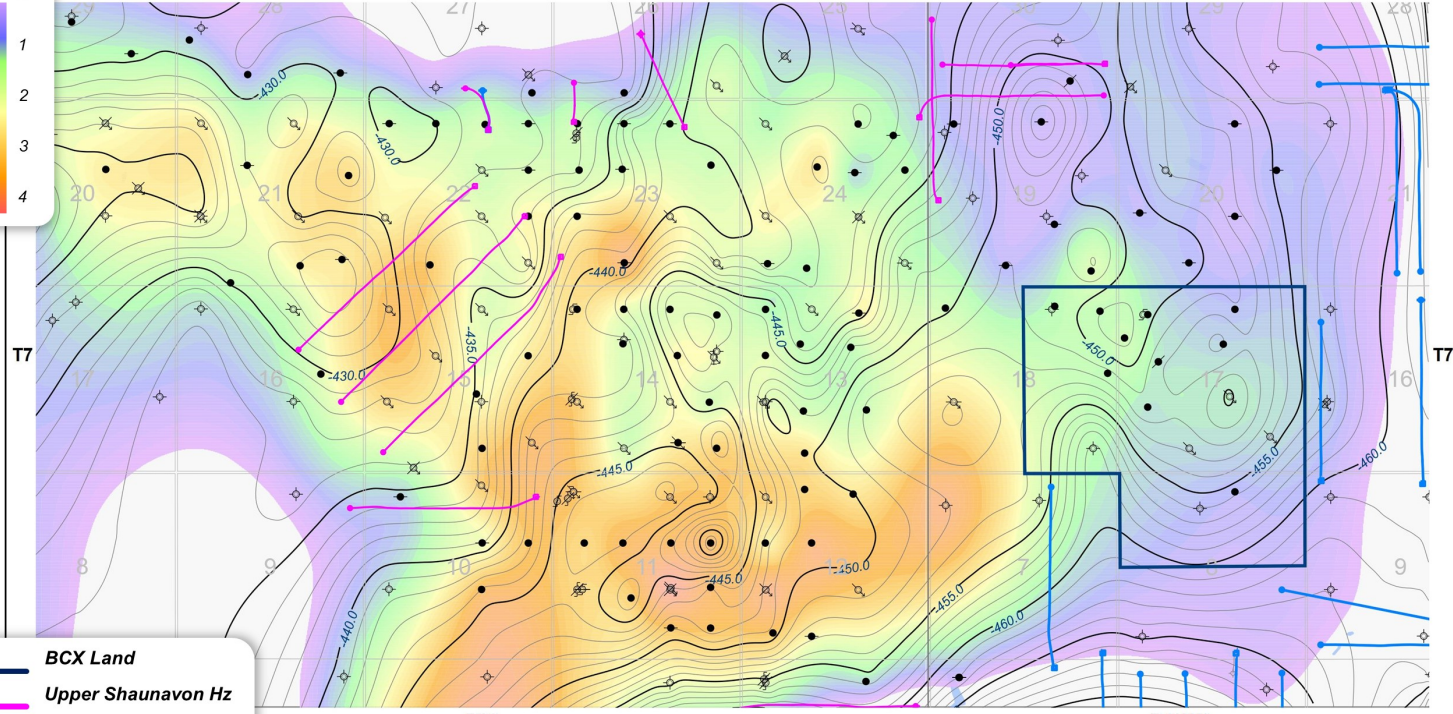
Dollard Upper Shaunavon Phi-H overlain by Upper Shaunavon structure (CI=1m)
