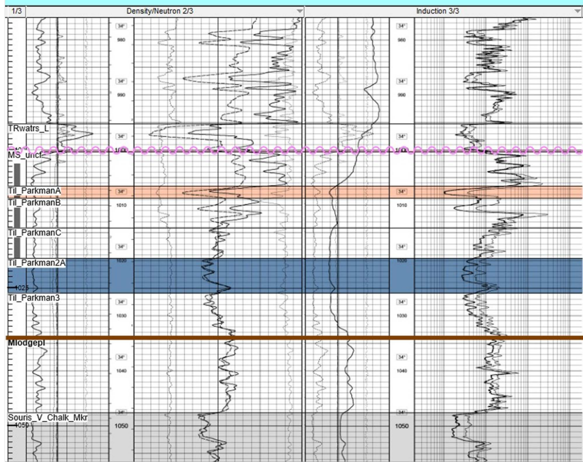
131/12-21-7-31W1 Tilston Type Log. Downdip well preserves all Parkman units before subcropping to the north
