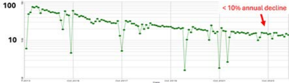
Production Plot (bbl/day) 01-02-76-11W6 Boundary Lake Perf
