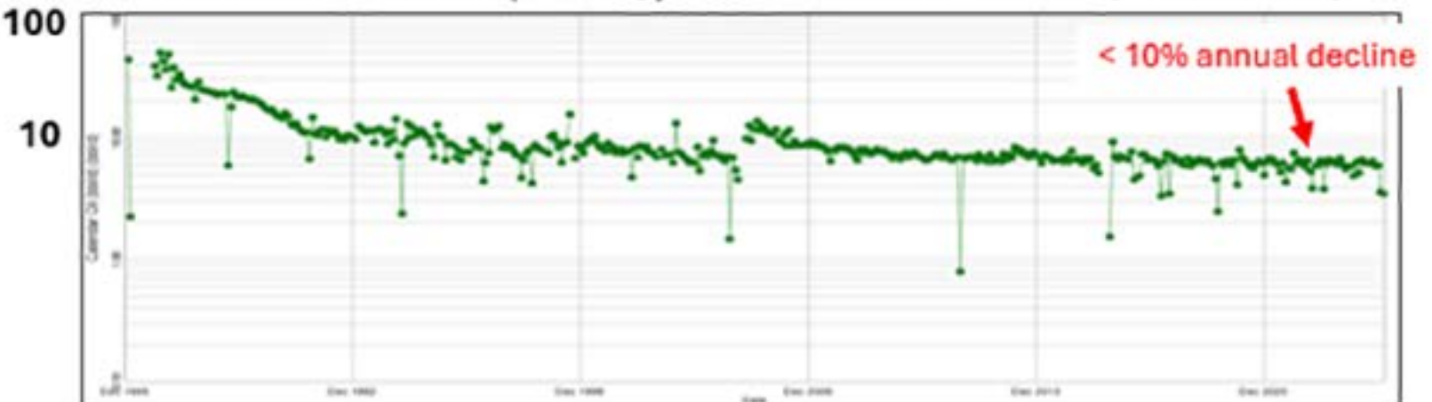
Flat Production Profile (bbl/day) 06-06-075-10W6/02 Boundary Lake Perf Only
