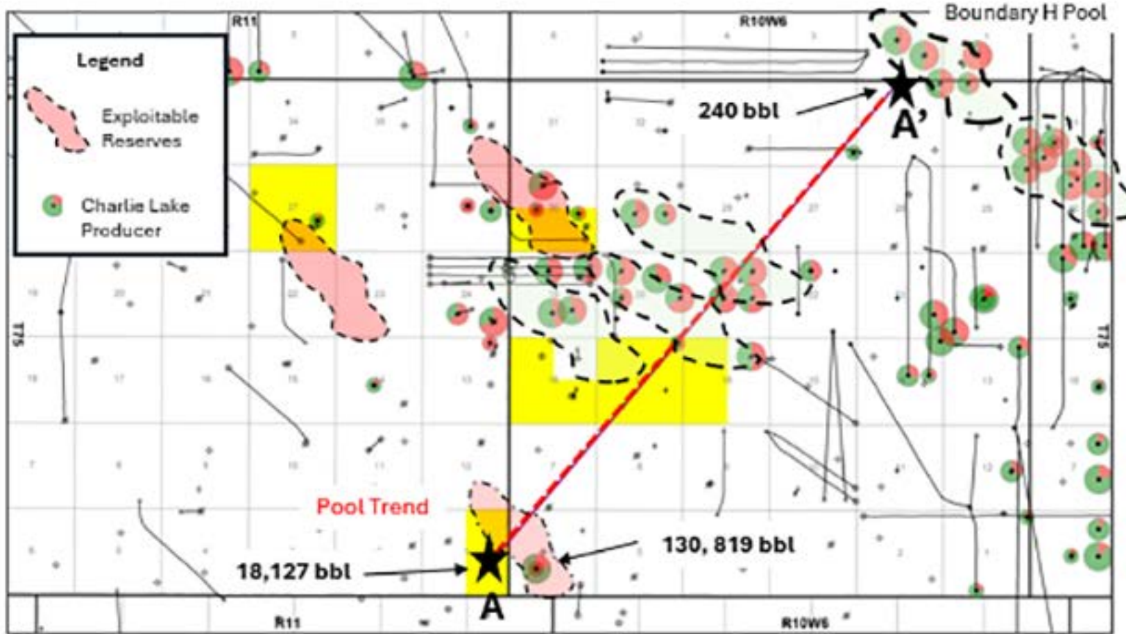
Boundary Cross Section A to A'
