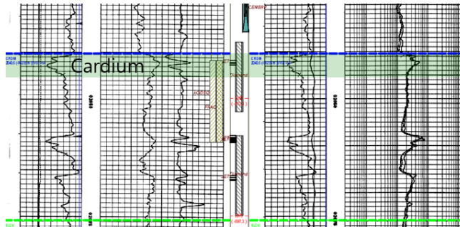
SOC Pine Ck 02/09-09-056-19W5/0 – Cardium Formation Log
